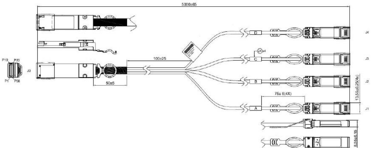
Mechanical Drawing
