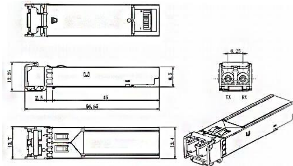
Mechanical Drawing
